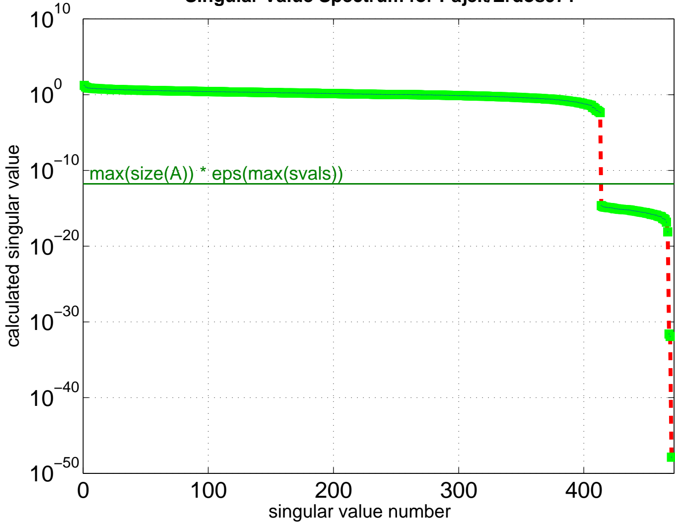
Singular Value Spectrum for Pajek/Erdos971
