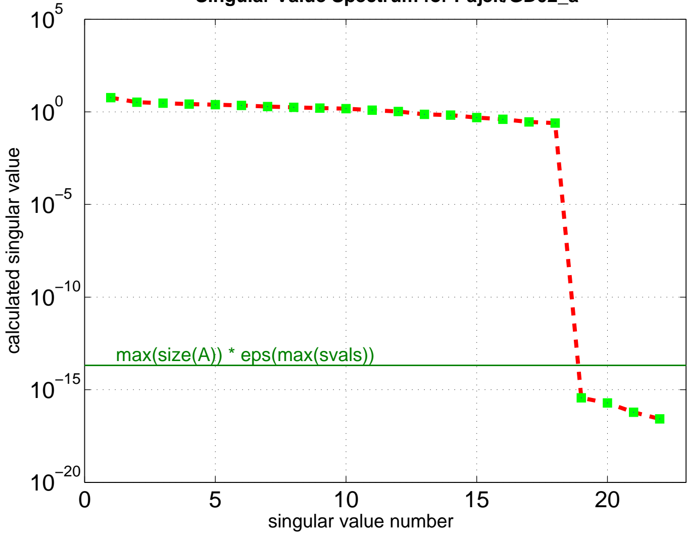
Singular Value Spectrum for Pajek/GD02_a
