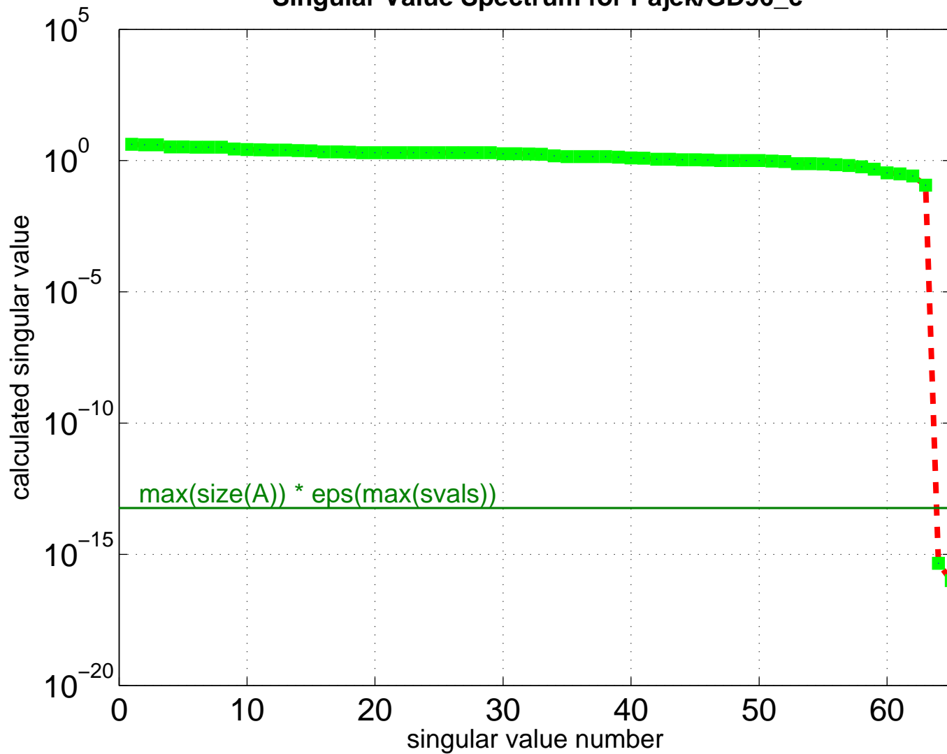
Singular Value Spectrum for Pajek/GD96_c
