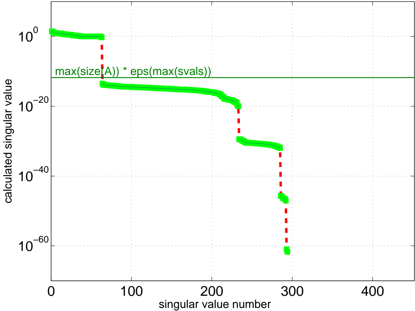
Singular Value Spectrum for Pajek/GD97_c
