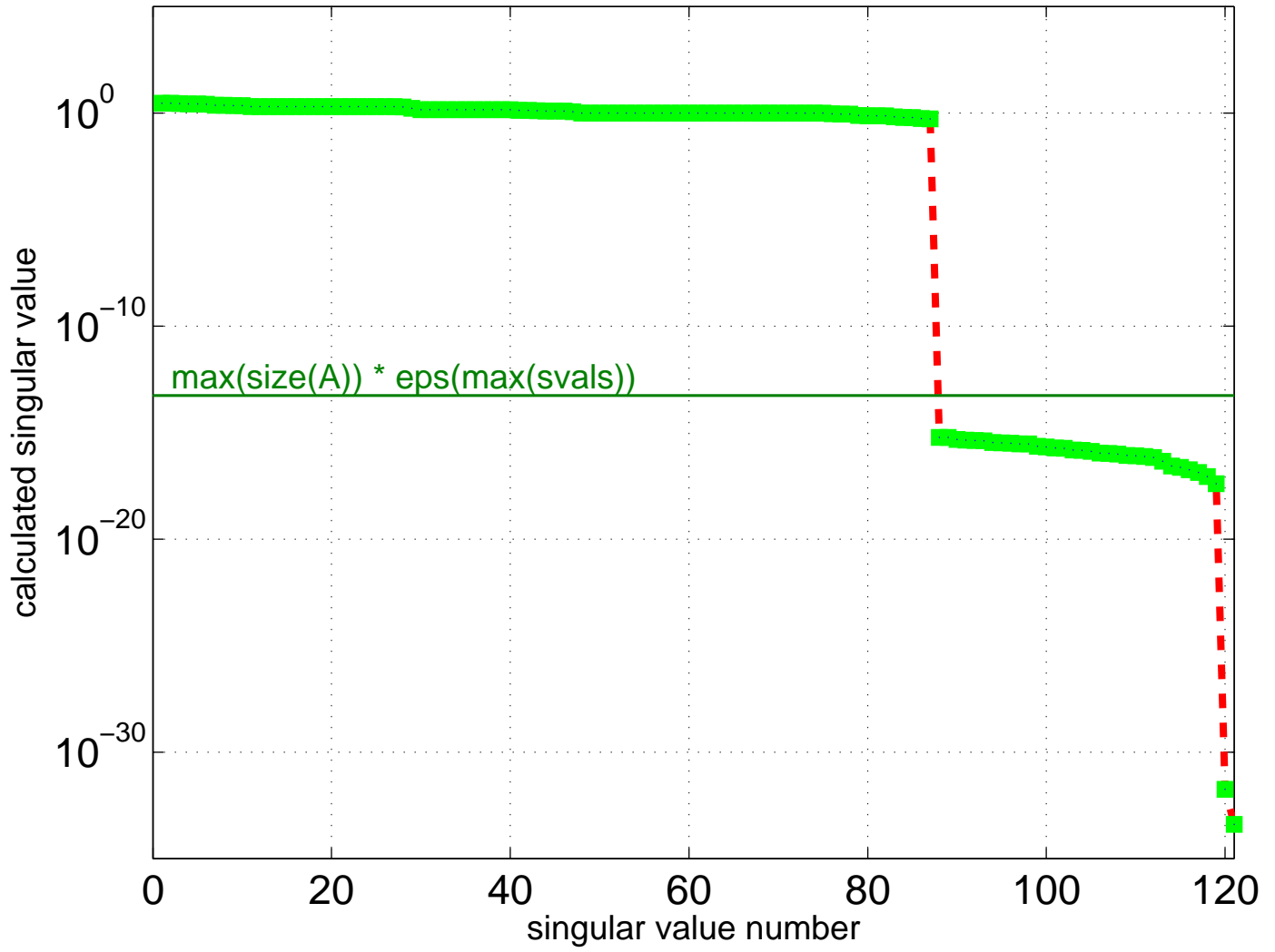
Singular Value Spectrum for Pajek/GD98_b
