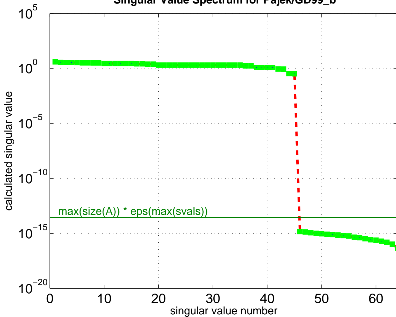
Singular Value Spectrum for Pajek/GD99_b
