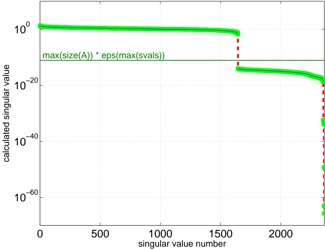
Singular Value Spectrum for Pajek/yeast
