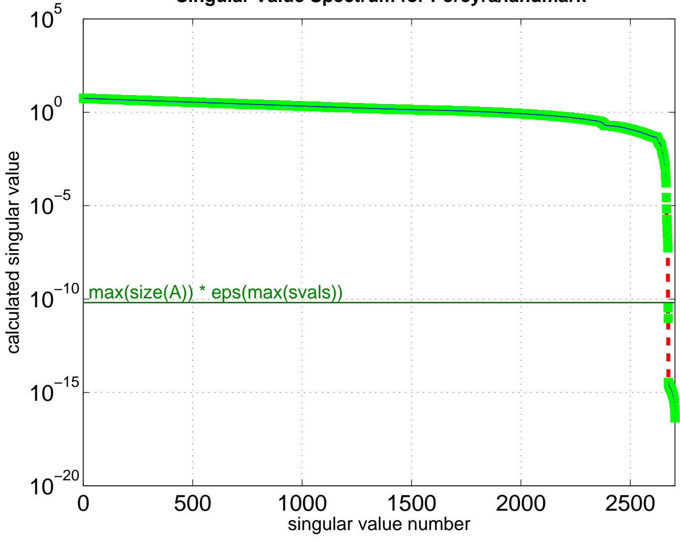
Singular Value Spectrum for Pereyra/landmark
