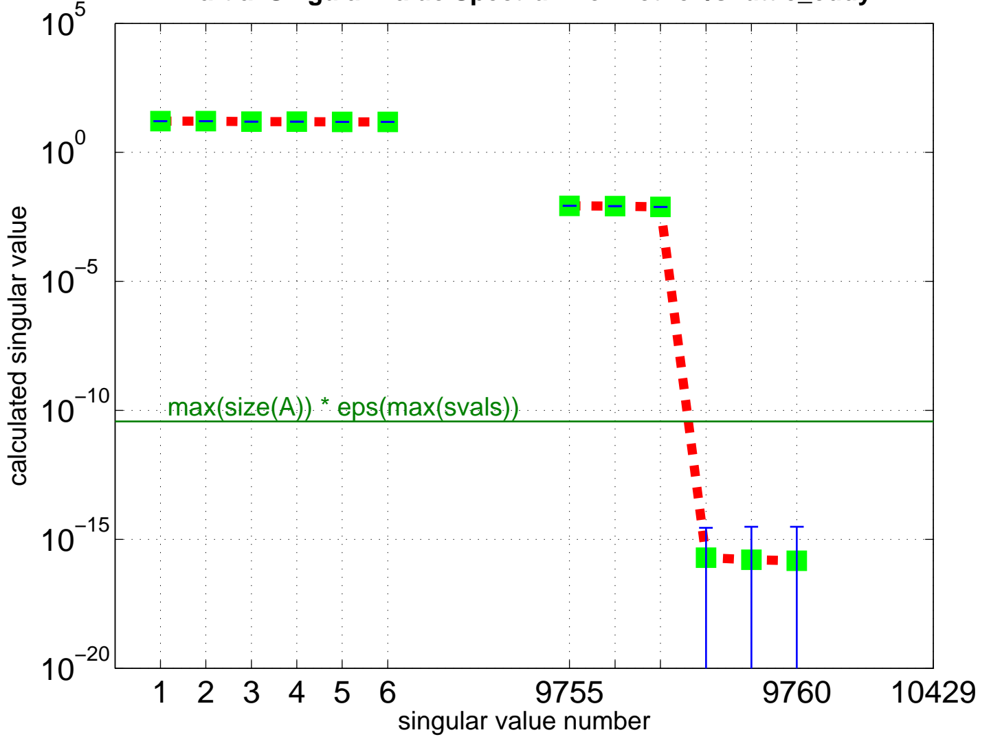
Partial Singular Value Spectrum for Pothen/shuttle_eddy
