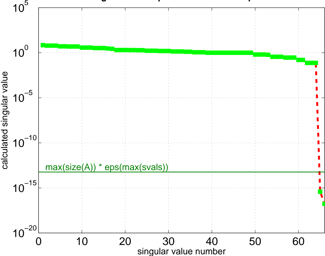
Singular Value Spectrum for Pothen/sphere2
