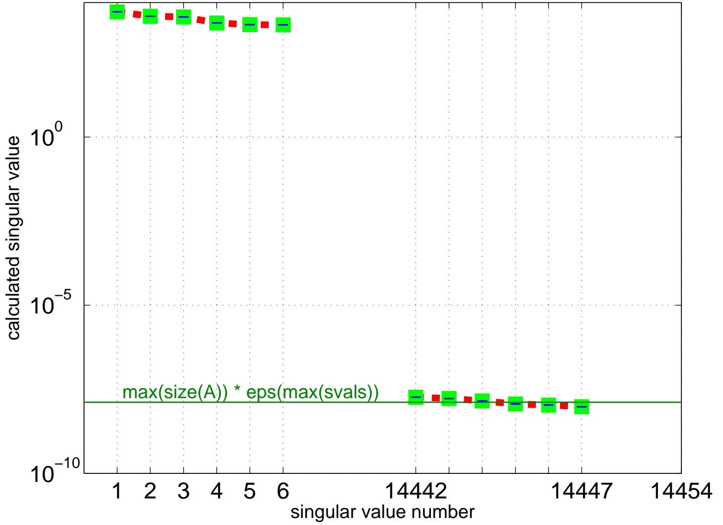
Partial Singular Value Spectrum for QY/case9
