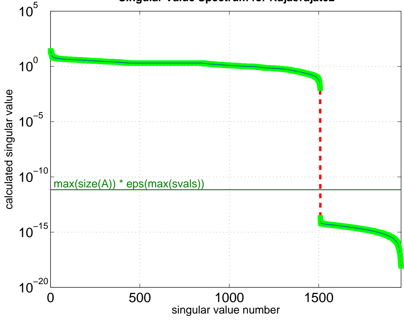
Singular Value Spectrum for Rajat/rajat02
