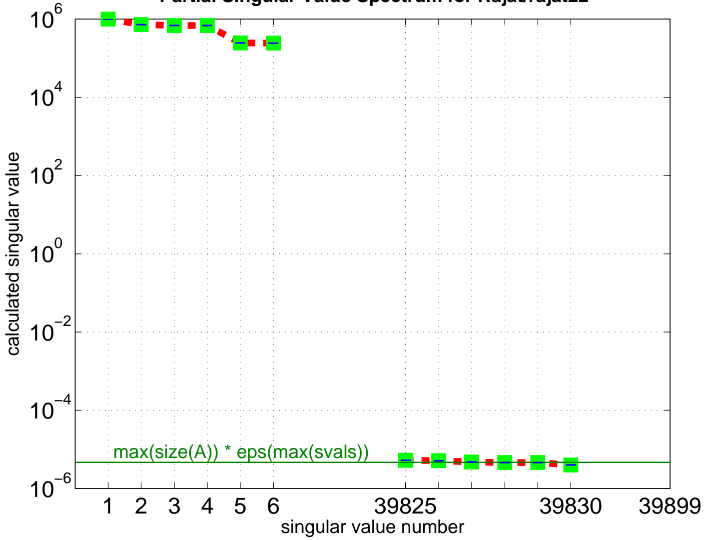
Partial Singular Value Spectrum for Rajat/rajat22
