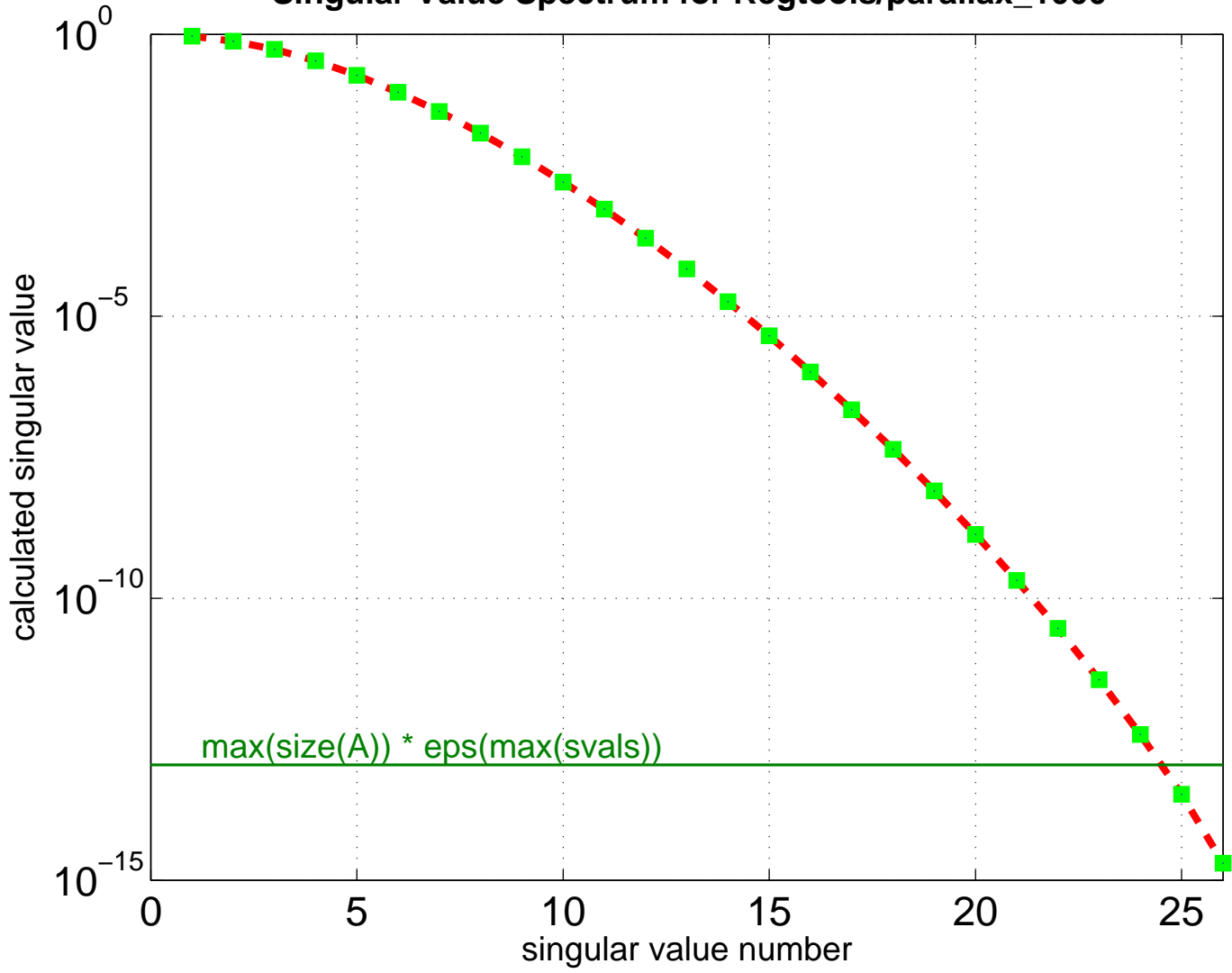
Singular Value Spectrum for Regtools/parallax_1000
