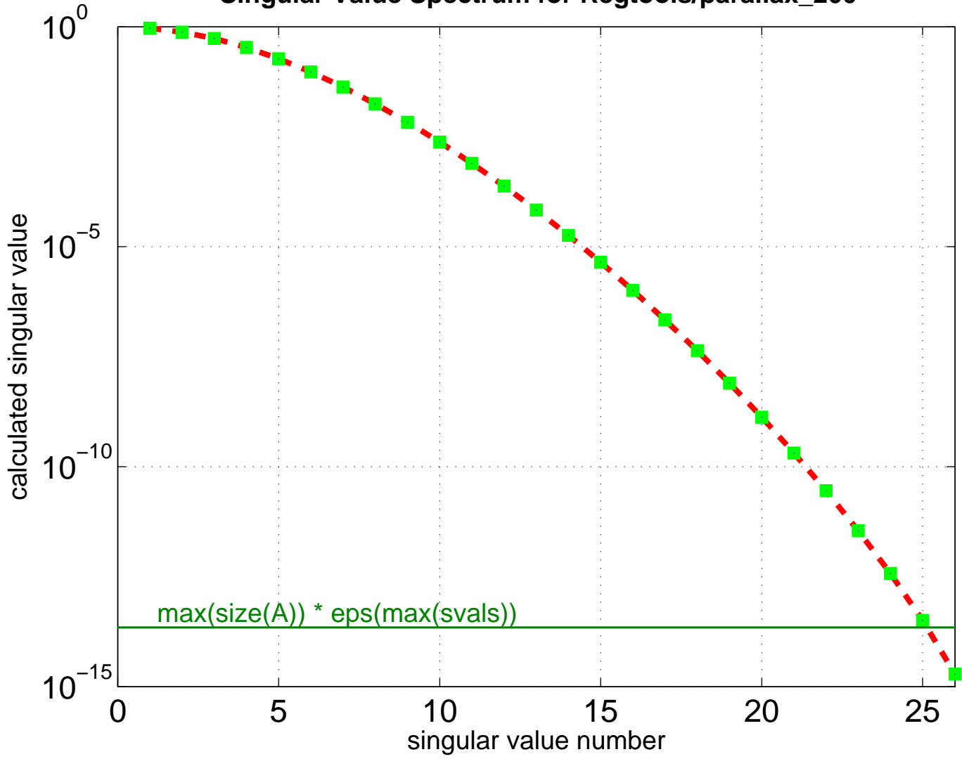
Singular Value Spectrum for Regtools/parallax_200
