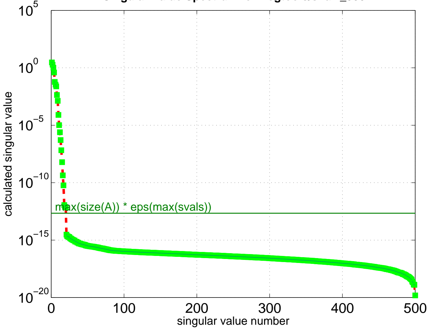
Singular Value Spectrum for Regtools/shaw_500
