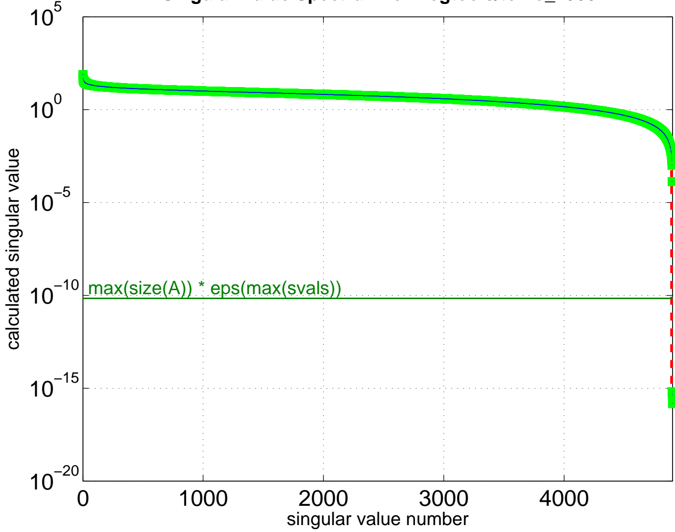
Singular Value Spectrum for Regtools/tomo_4900
