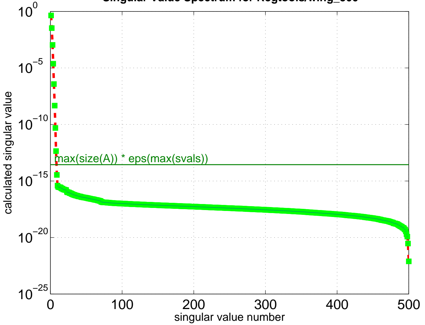
Singular Value Spectrum for Regtools/wing_500
