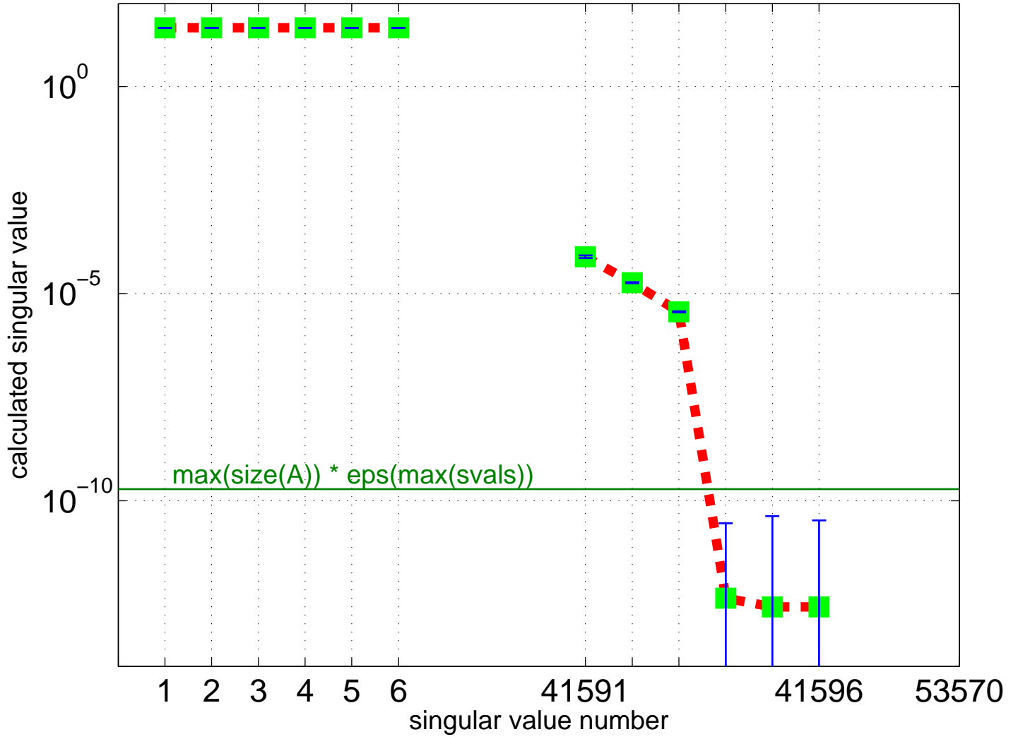
Partial Singular Value Spectrum for Rothberg/struct3
