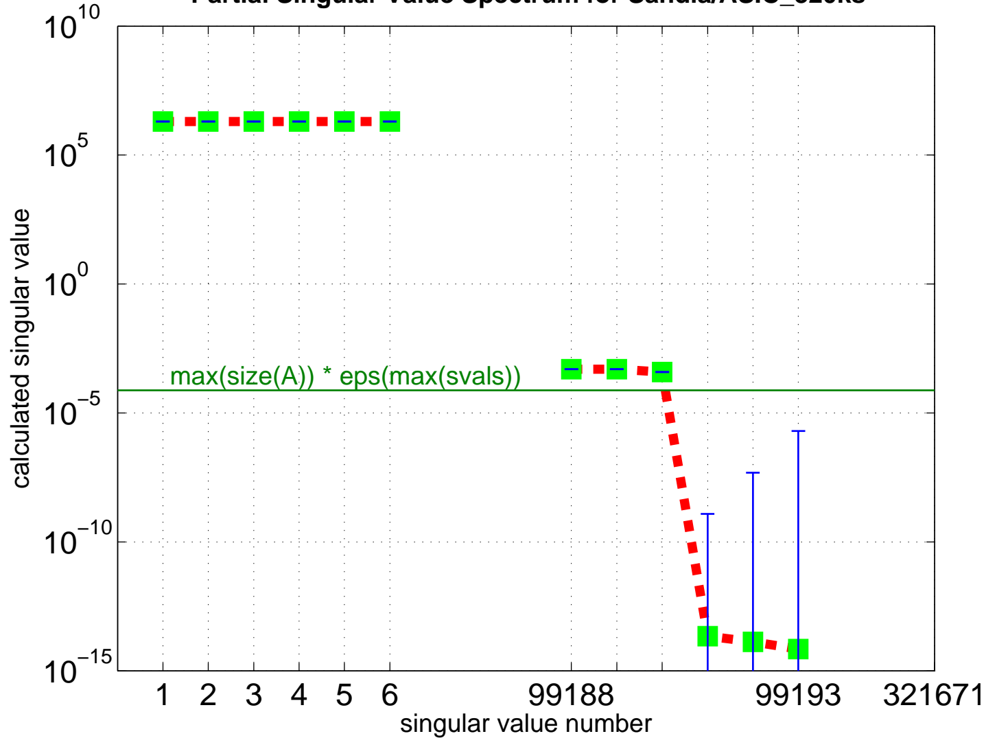
Partial Singular Value Spectrum for Sandia/ASIC_320ks
