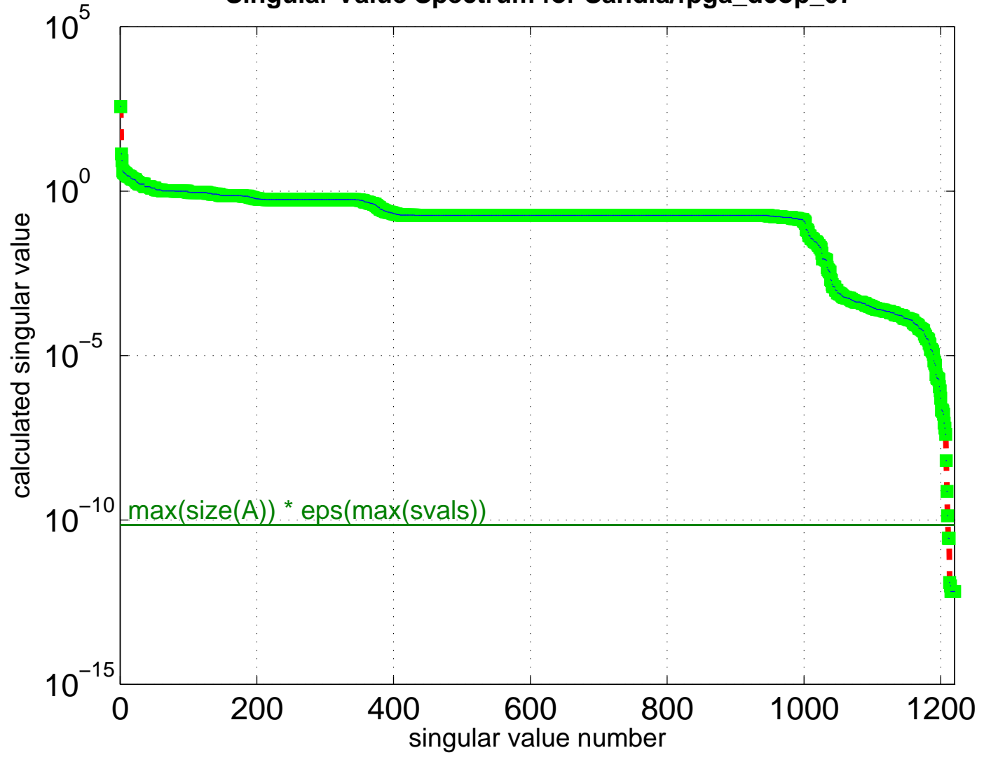
Singular Value Spectrum for Sandia/fpga_dcop_07
