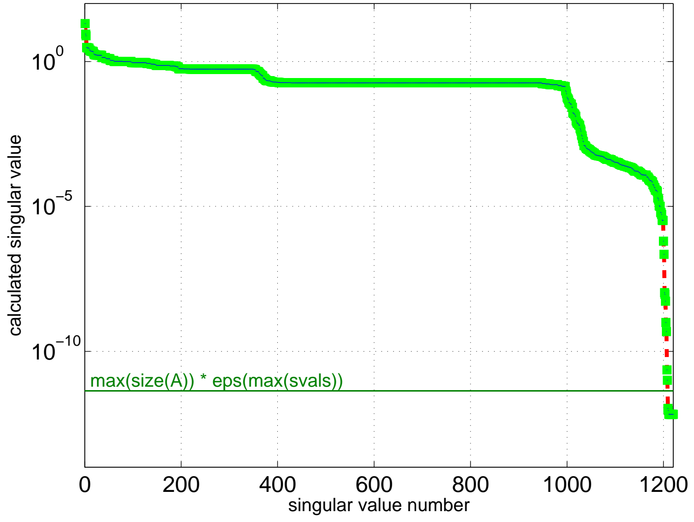
Singular Value Spectrum for Sandia/fpga_dcop_09
