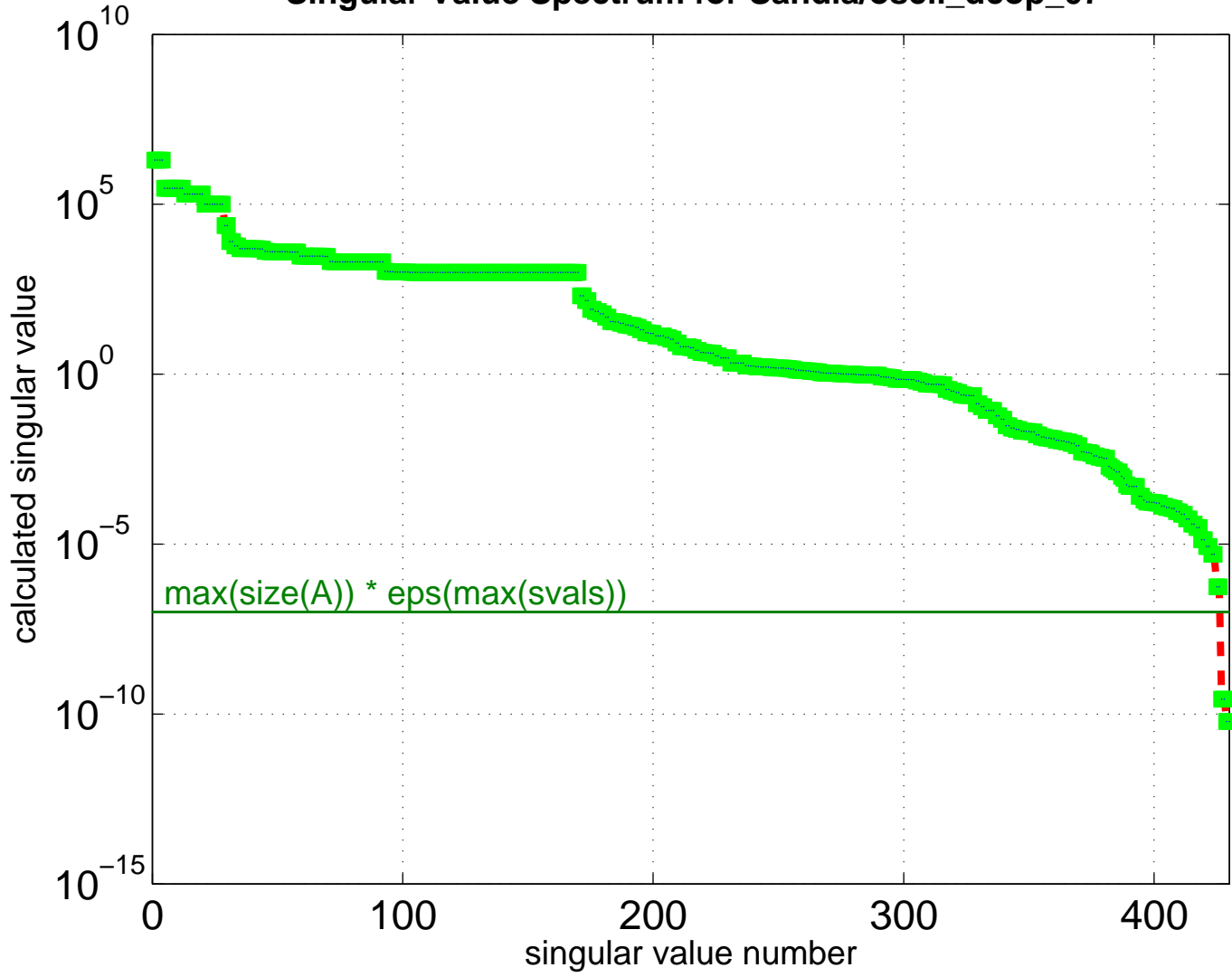
Singular Value Spectrum for Sandia/oscil_dcop_07
