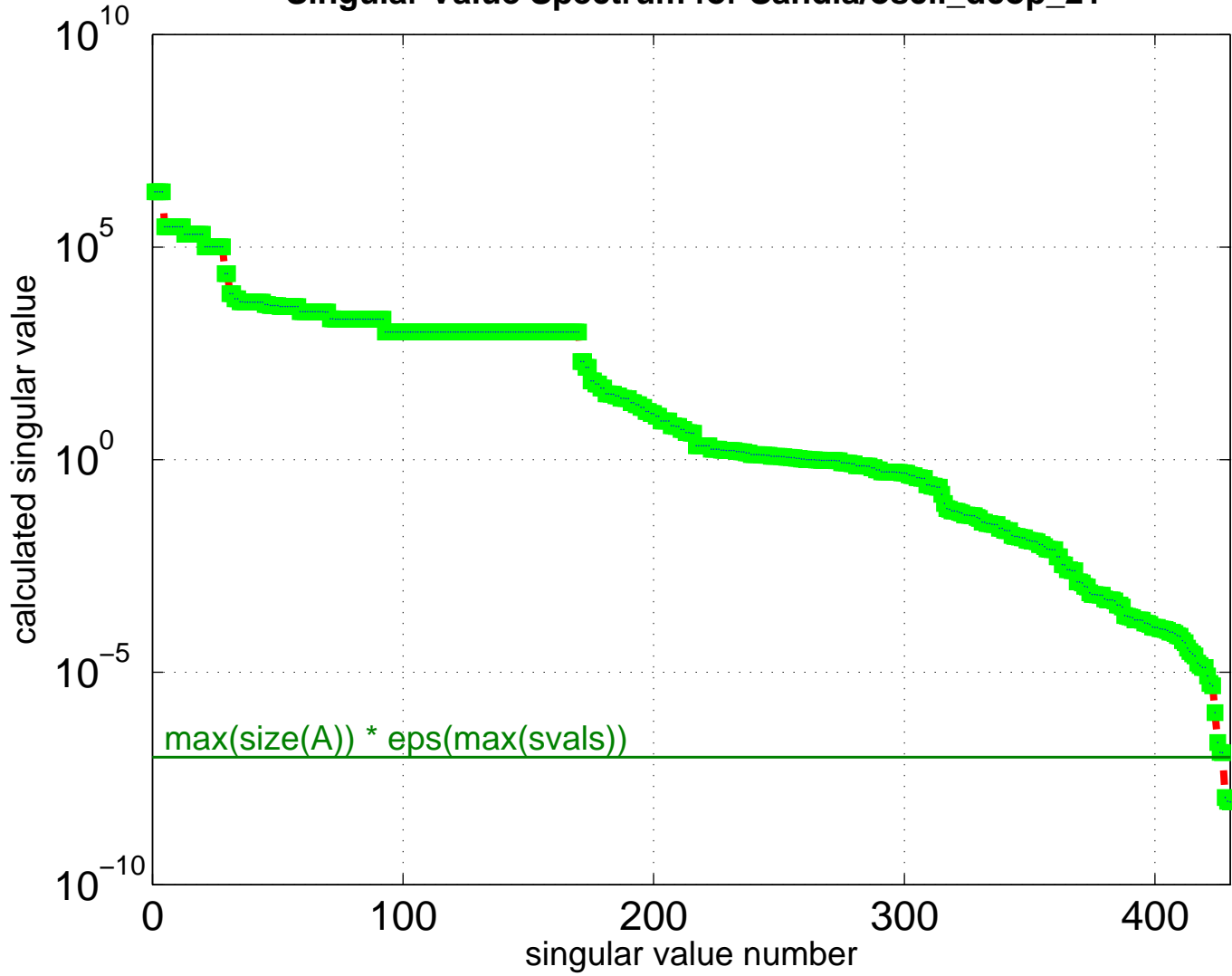
Singular Value Spectrum for Sandia/oscil_dcop_21
