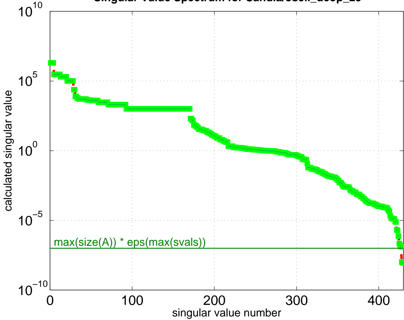
Singular Value Spectrum for Sandia/oscil_dcop_25
