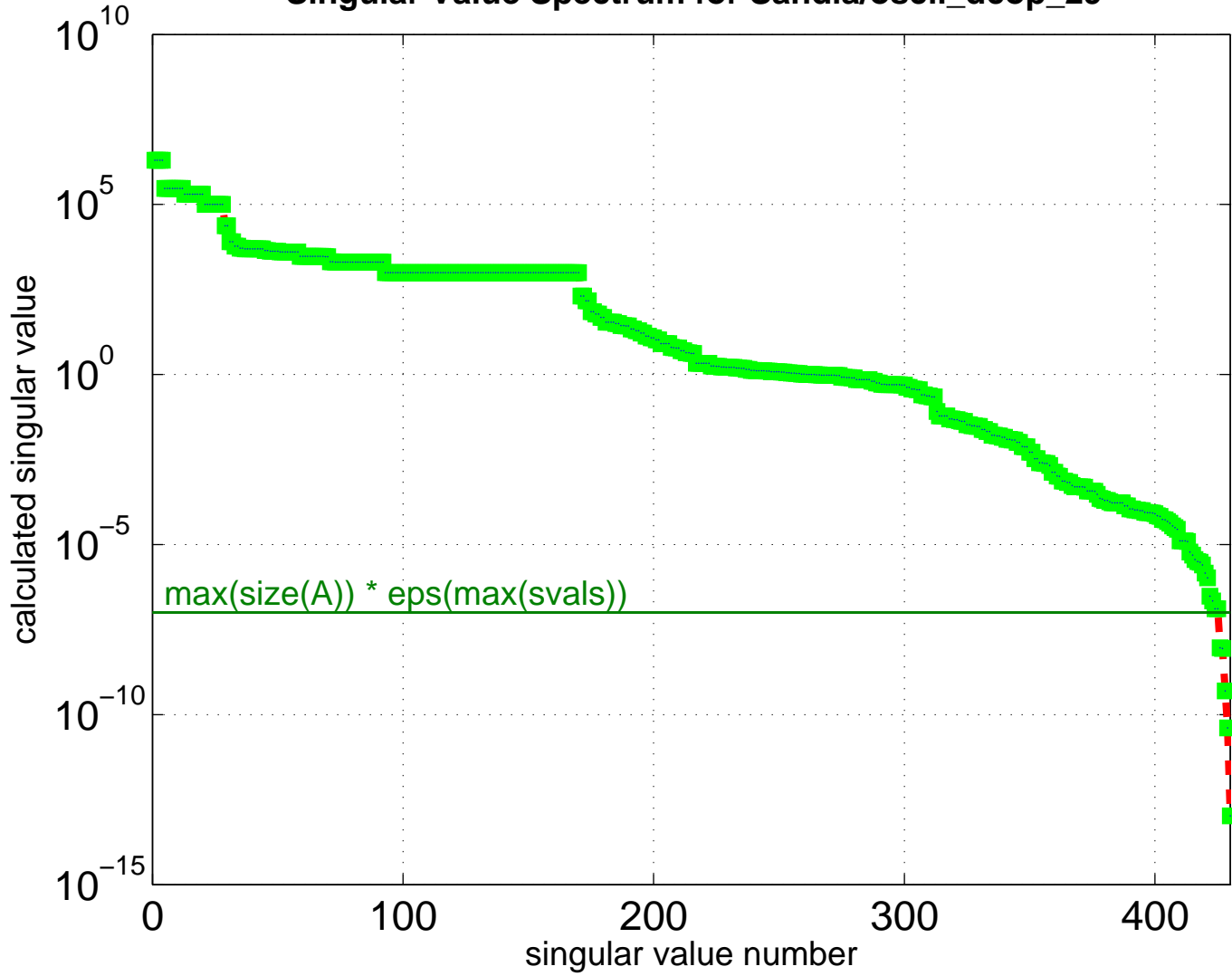
Singular Value Spectrum for Sandia/oscil_dcop_29
