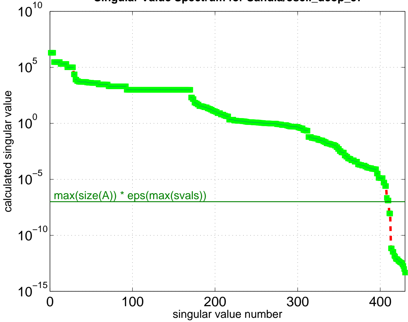
Singular Value Spectrum for Sandia/oscil_dcop_57
