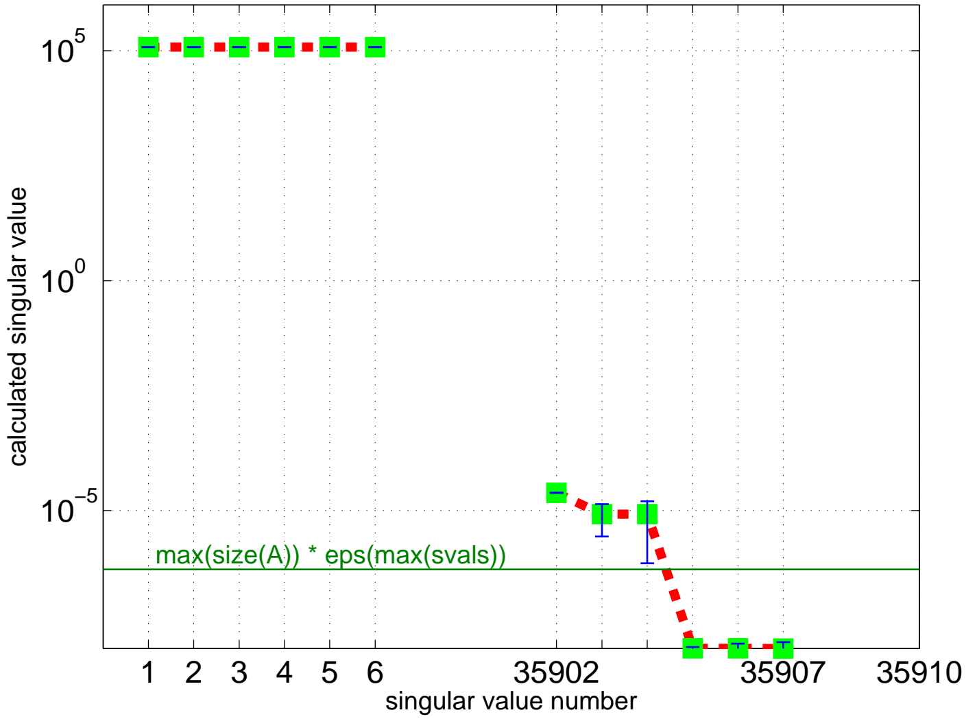
Partial Singular Value Spectrum for Schenk_IBMNA/c-56
