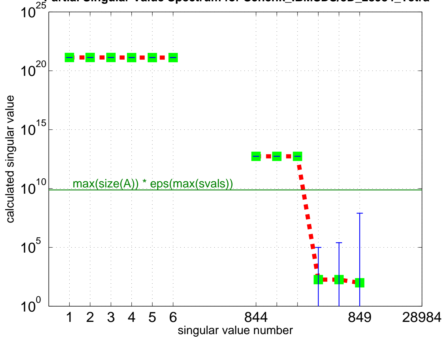
Partial Singular Value Spectrum for Schenk_IBMSDS/3D_28984_Tetra
