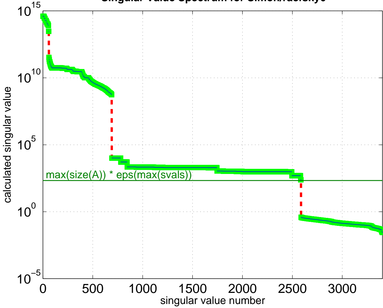
Singular Value Spectrum for Simon/raefsky6
