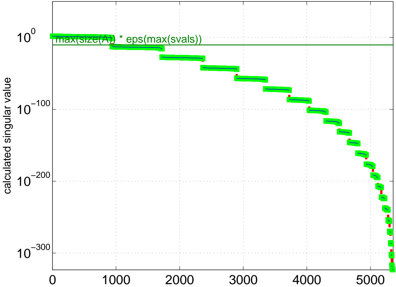
Singular Value Spectrum for TKK/g3rmt3m3
