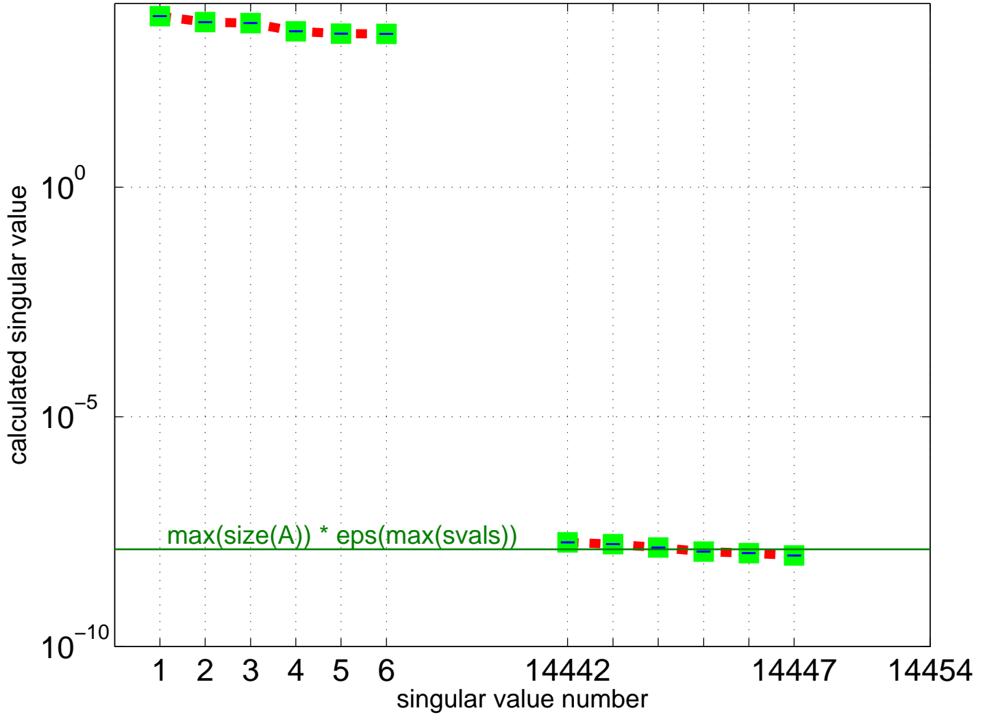
Partial Singular Value Spectrum for TSOPF/TSOPF_FS_b9_c6
