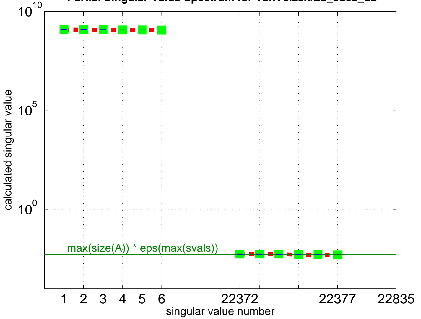
Partial Singular Value Spectrum for VanVelzen/Zd_Jac3_db
