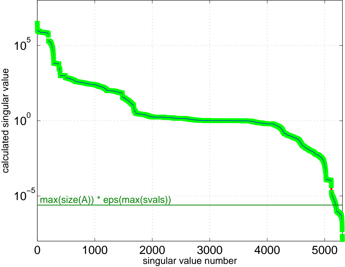
Singular Value Spectrum for Zitney/hydr1c
