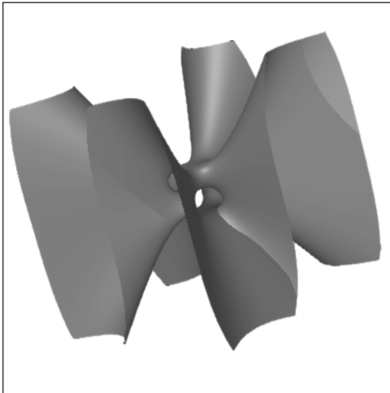
FIGURE 1. Quartic surface.
